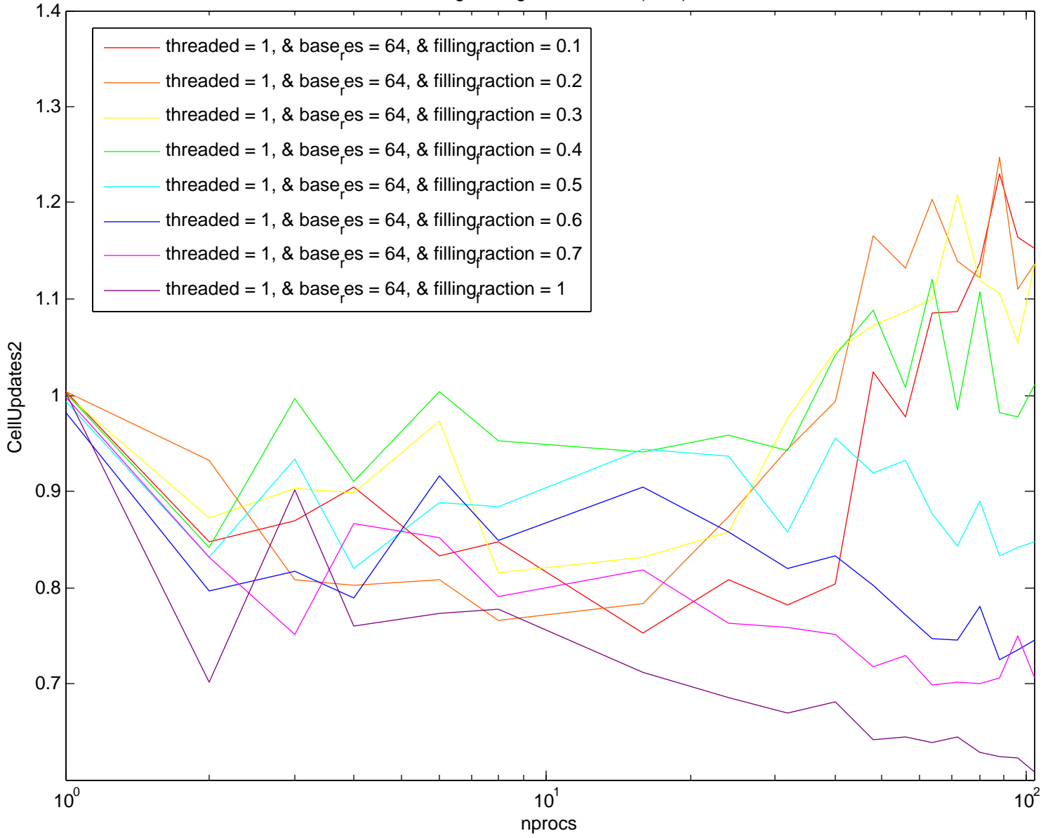
StrongScalingThreadRatios(-1/0)
